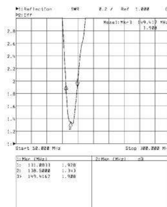
V.S.W.R. CURVE
