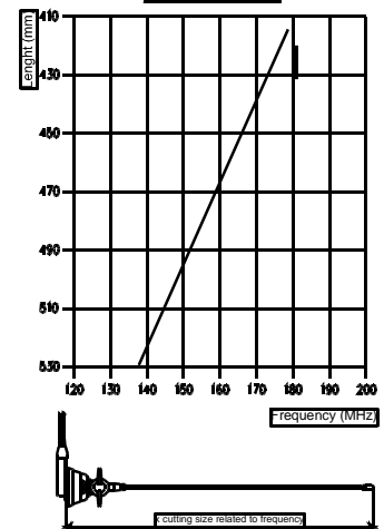
Cutting Diagram
