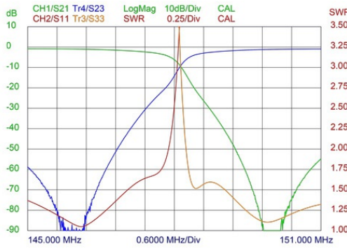
Typical response curves @ 4 MHz duplex spacing
